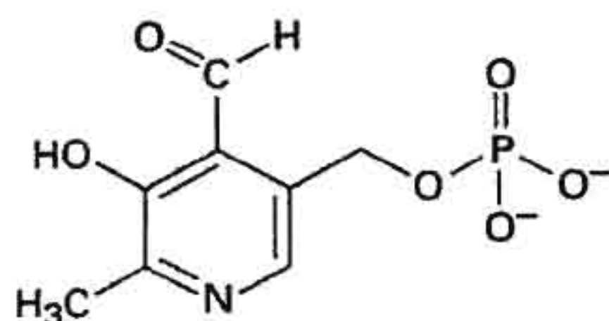
Pyridoxal phosphate
